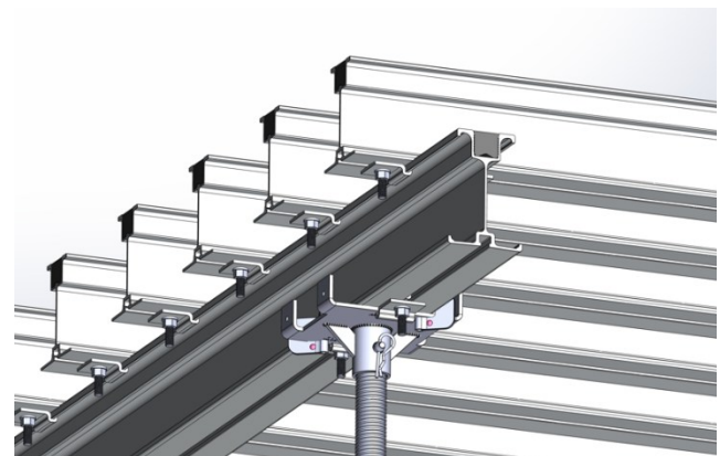
Al beam Clamping with FOUR WAY U-HEAD (FOR SCREW)
