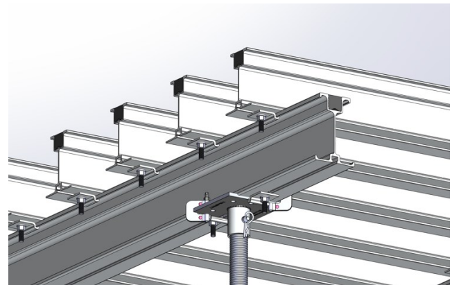
Al beam Clamping with BASE PLATE (FOR SCREW)
